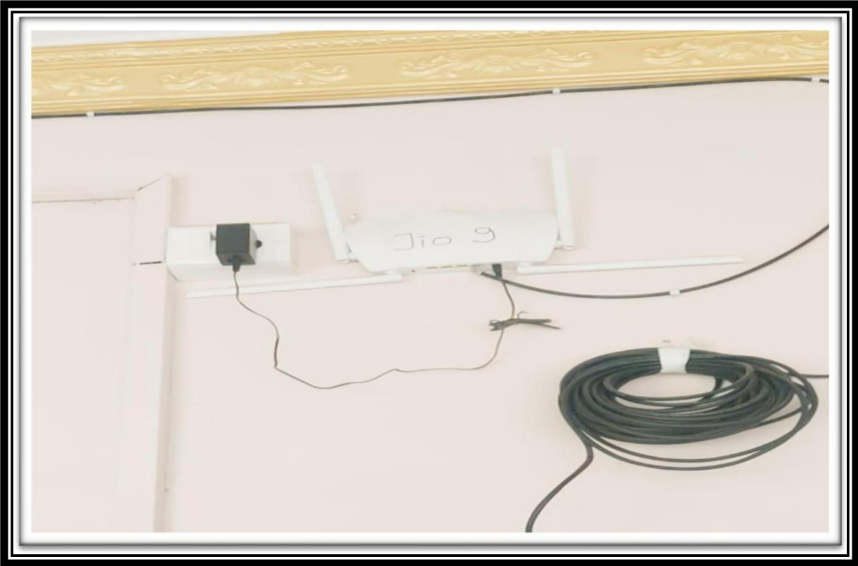
WithRouter:
